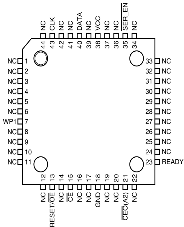
44-lead TQFP
